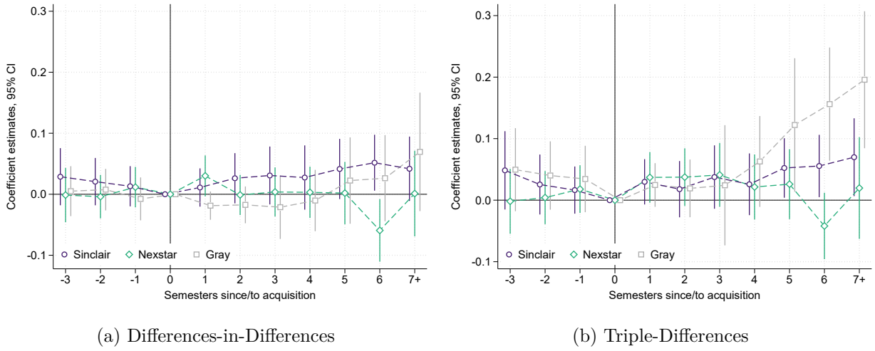
Figure A8: Effect of Group Ownership on Impressions, Event Studies
