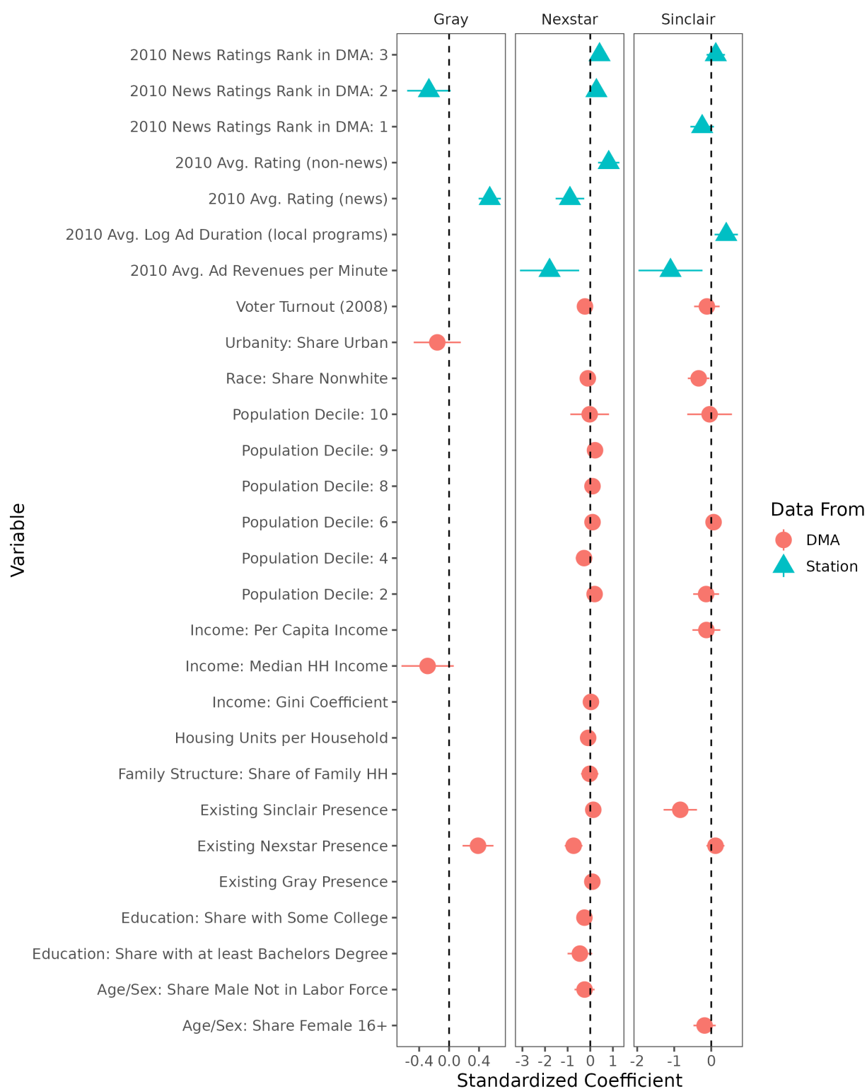
Figure D1: Model estimates from L1-penalized logistic regression of an indicator for acquisition by each of the three large groups on station- and media-market-level characteristics.
